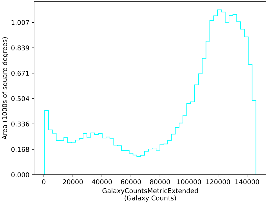
ddf_loaded_half_fl1_v3.3_10yrs u: GalaxyCountsMetricExtended
