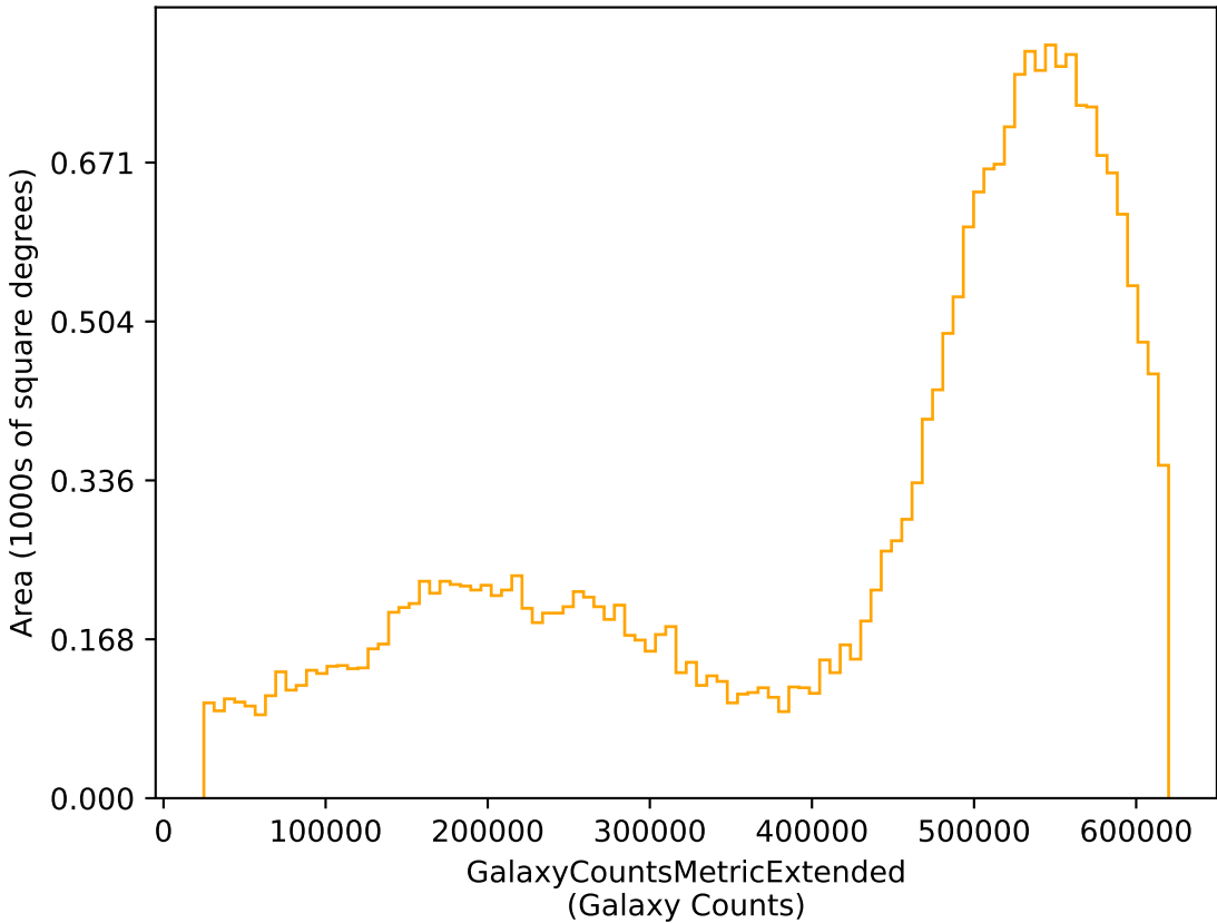
ddf_loaded_half_fl1_v3.3_10yrs r: GalaxyCountsMetricExtended
