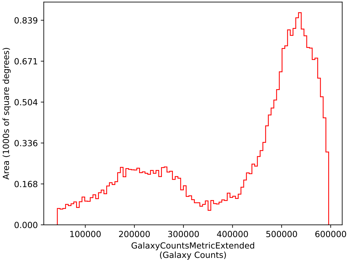
ddf_loaded_half_fl1_v3.3_10yrs i: GalaxyCountsMetricExtended
