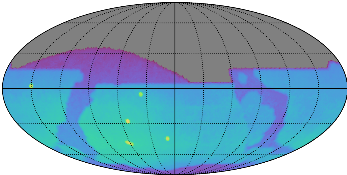
ddf_loaded_half_fl1_v3.3_10yrs : Brown Dwarf, L7
