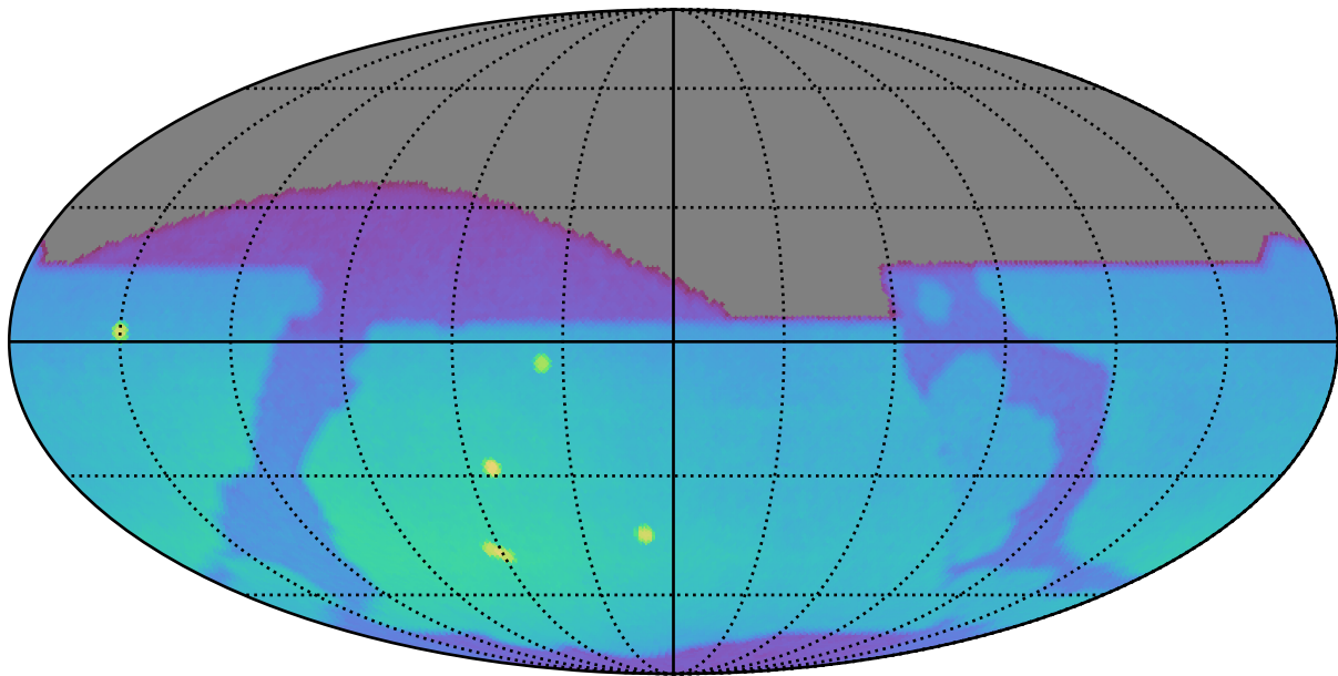
ddf_loaded_half_fl1_v3.3_10yrs : Brown Dwarf, L4
