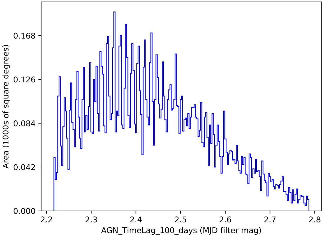
ddf_loaded_half_fl1_v3.3_10yrs y band: AGN_TimeLag_100_days
