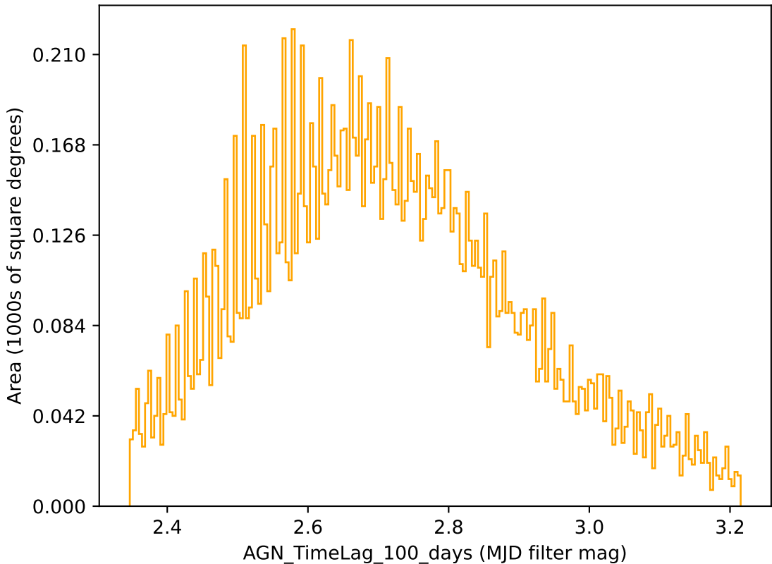
ddf_loaded_half_fl1_v3.3_10yrs r band: AGN_TimeLag_100_days
