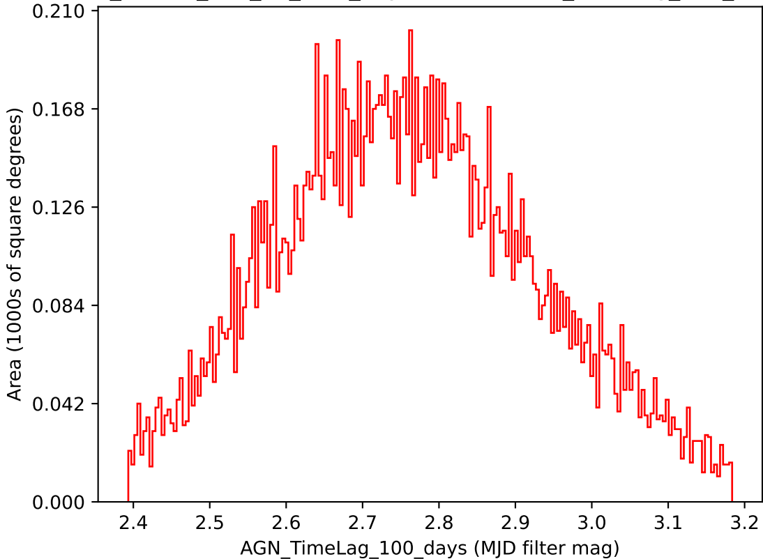
ddf_loaded_half_fl1_v3.3_10yrs i band: AGN_TimeLag_100_days
