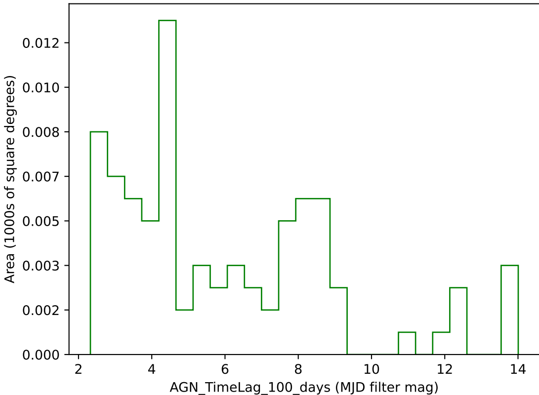
ddf_loaded_half_fl1_v3.3_10yrs g band: AGN_TimeLag_100_days
