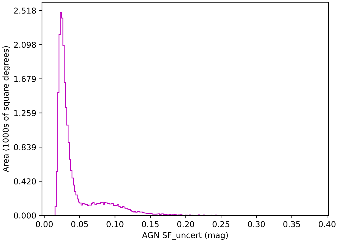
ddf_loaded_half_fl1_v3.3_10yrs z band: AGN SF_uncert
