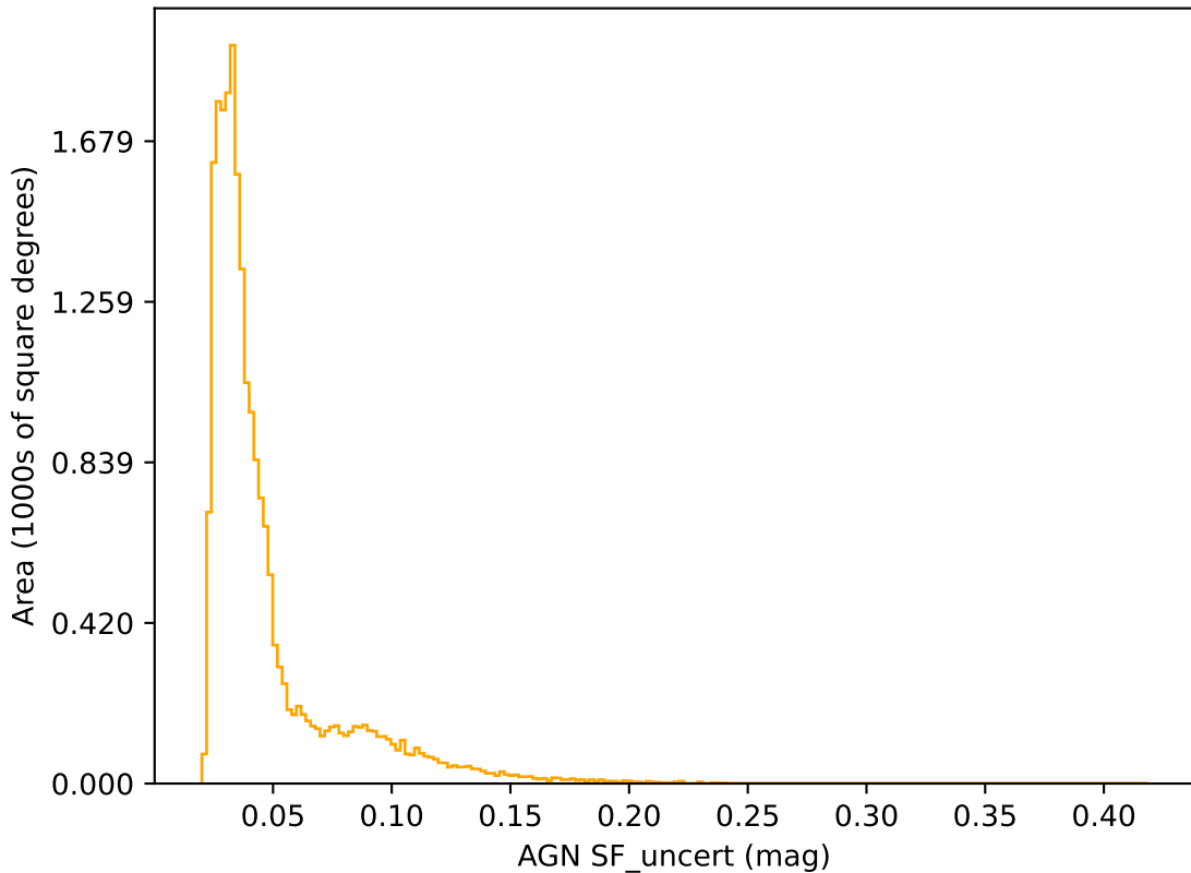
ddf_loaded_half_fl1_v3.3_10yrs r band: AGN SF_uncert
