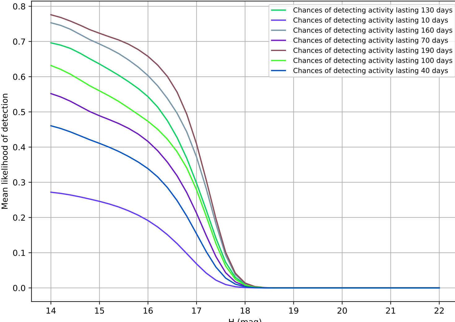
ddf loaded half fl15 v3.4 10yrs Trojan
