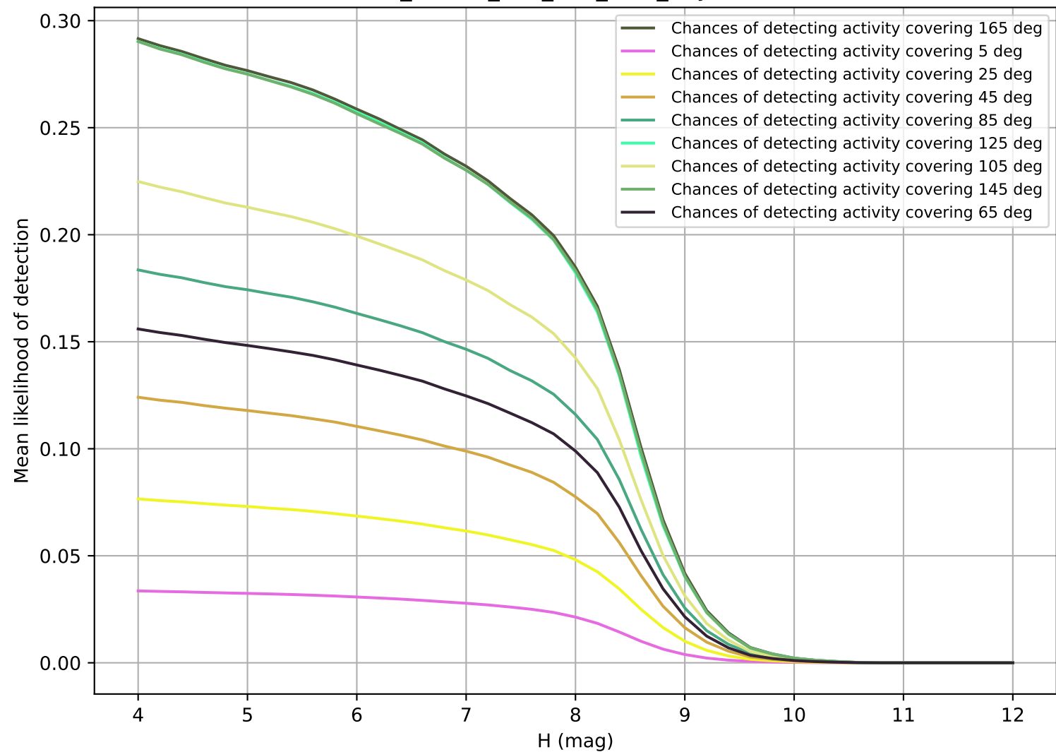
ddf_loaded_half_fl15_v3.4_10yrs TNO
