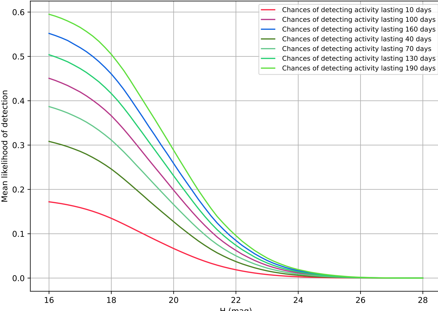
ddf loaded half fl15 v3.4 10yrs NEO
