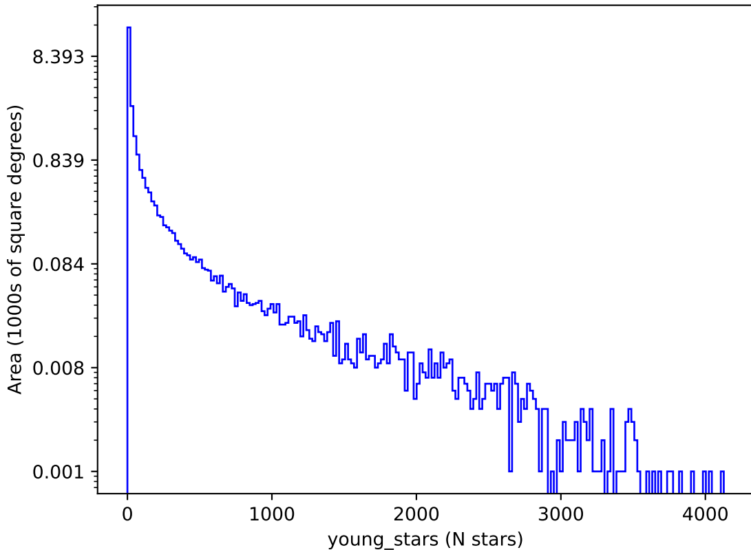
ddf_loaded_half_fl15_v3.4_10yrs : young_stars
