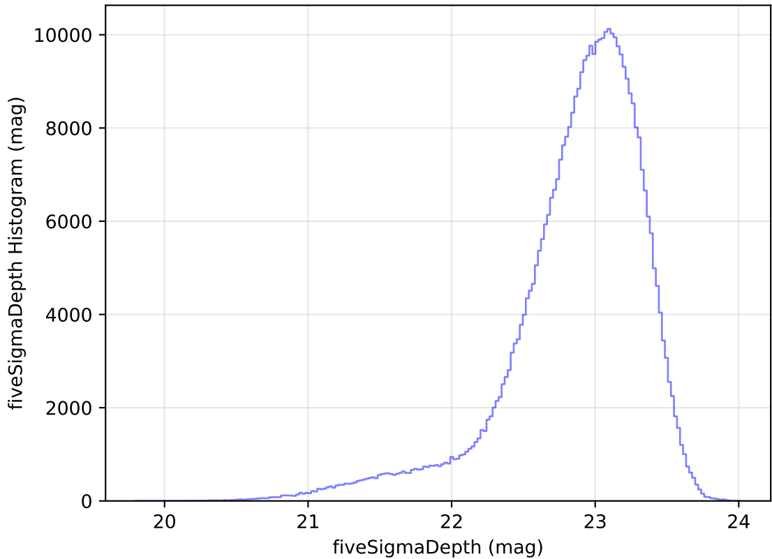
ddf_loaded_half_fl15_v3.4_10yrs z: fiveSigmaDepth Histogram
