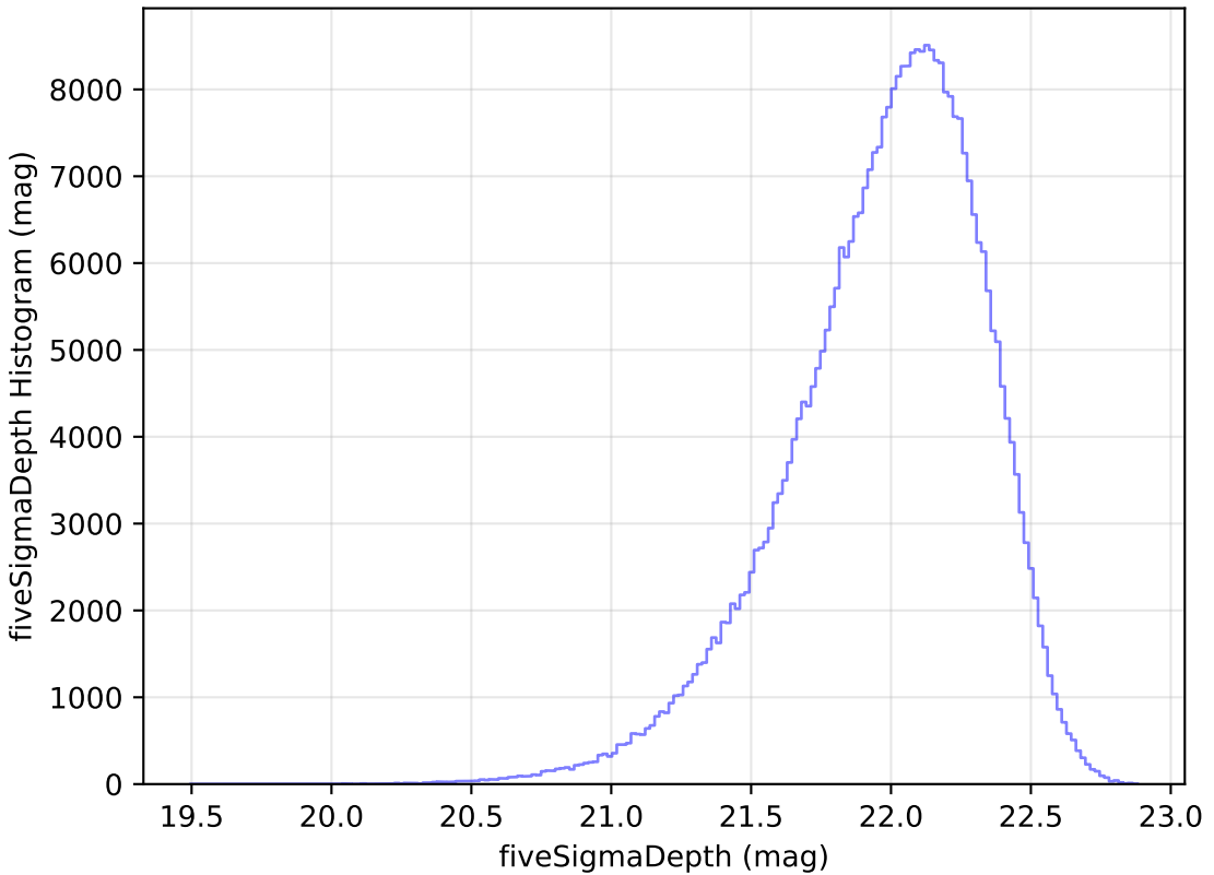
ddf_loaded_half_fl15_v3.4_10yrs y: fiveSigmaDepth Histogram
