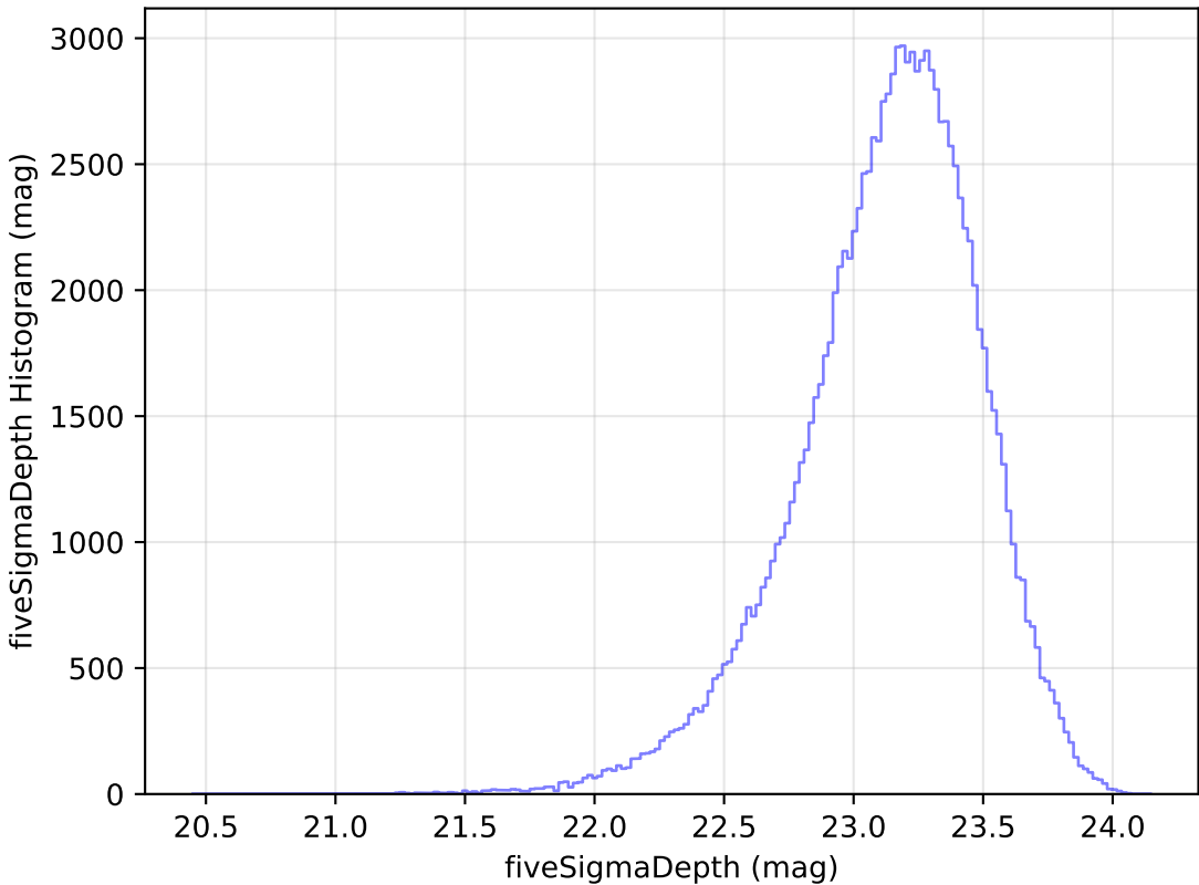
ddf_loaded_half_fl15_v3.4_10yrs u: fiveSigmaDepth Histogram
