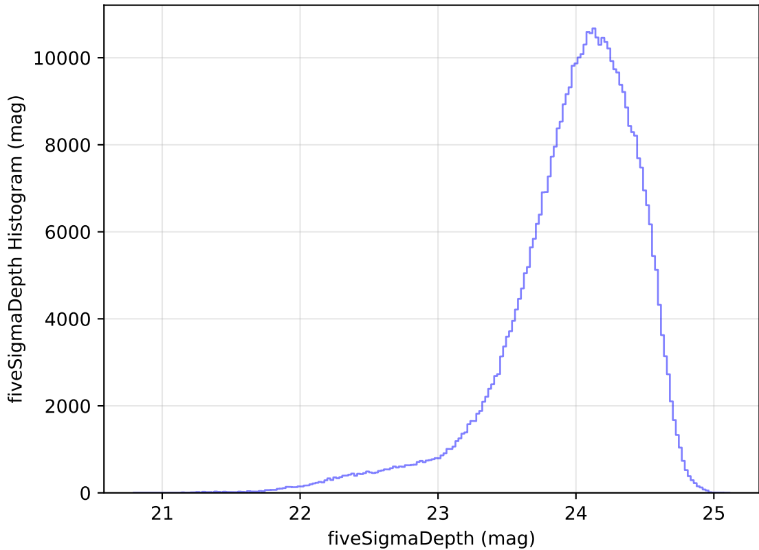
ddf_loaded_half_fl15_v3.4_10yrs r: fiveSigmaDepth Histogram
