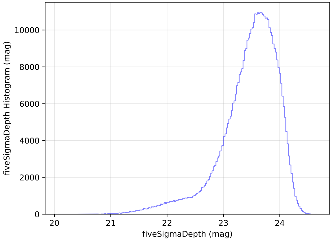
ddf_loaded_half_fl15_v3.4_10yrs i: fiveSigmaDepth Histogram
