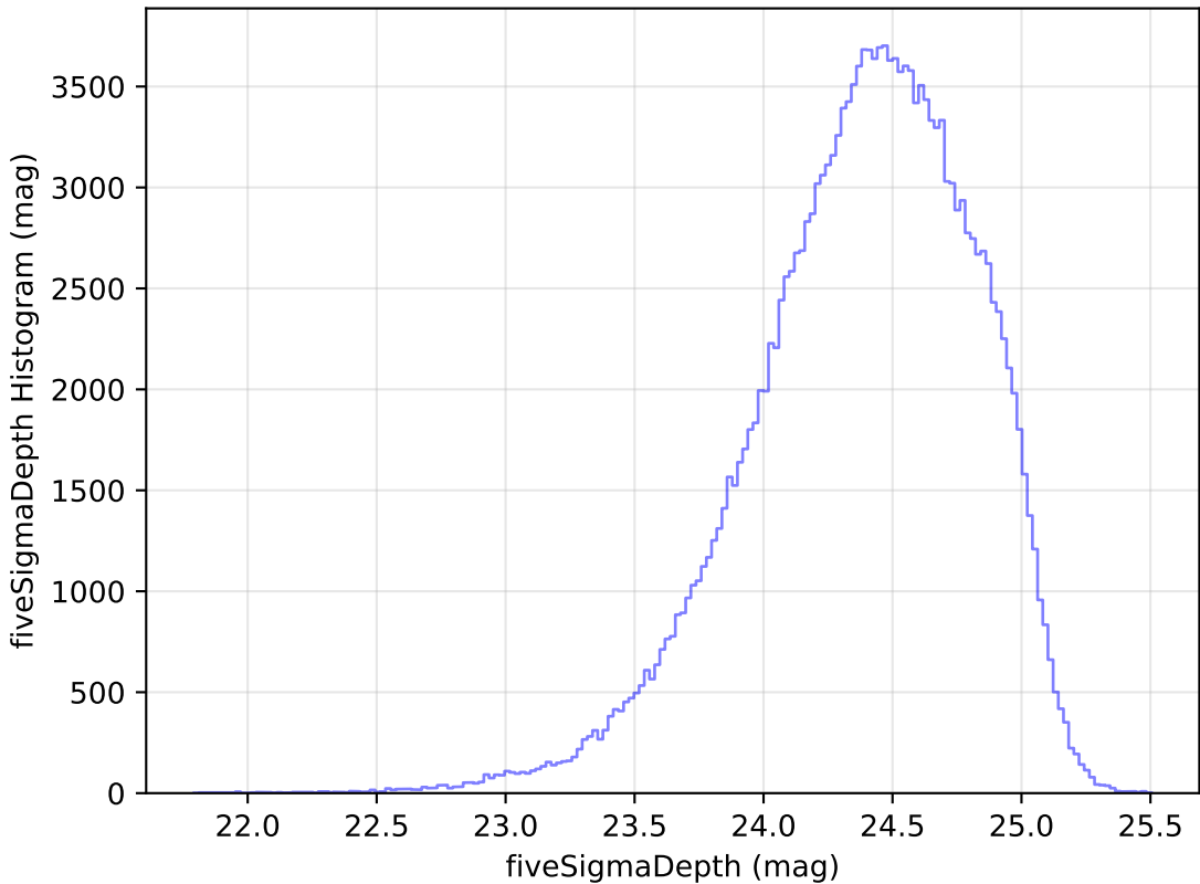
ddf_loaded_half_fl15_v3.4_10yrs g: fiveSigmaDepth Histogram
