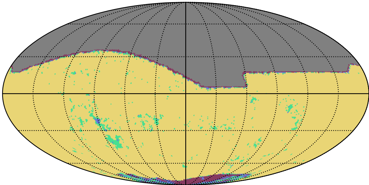
ddf_loaded_half_fl15_v3.4_10yrs r band: YearCoverage night
