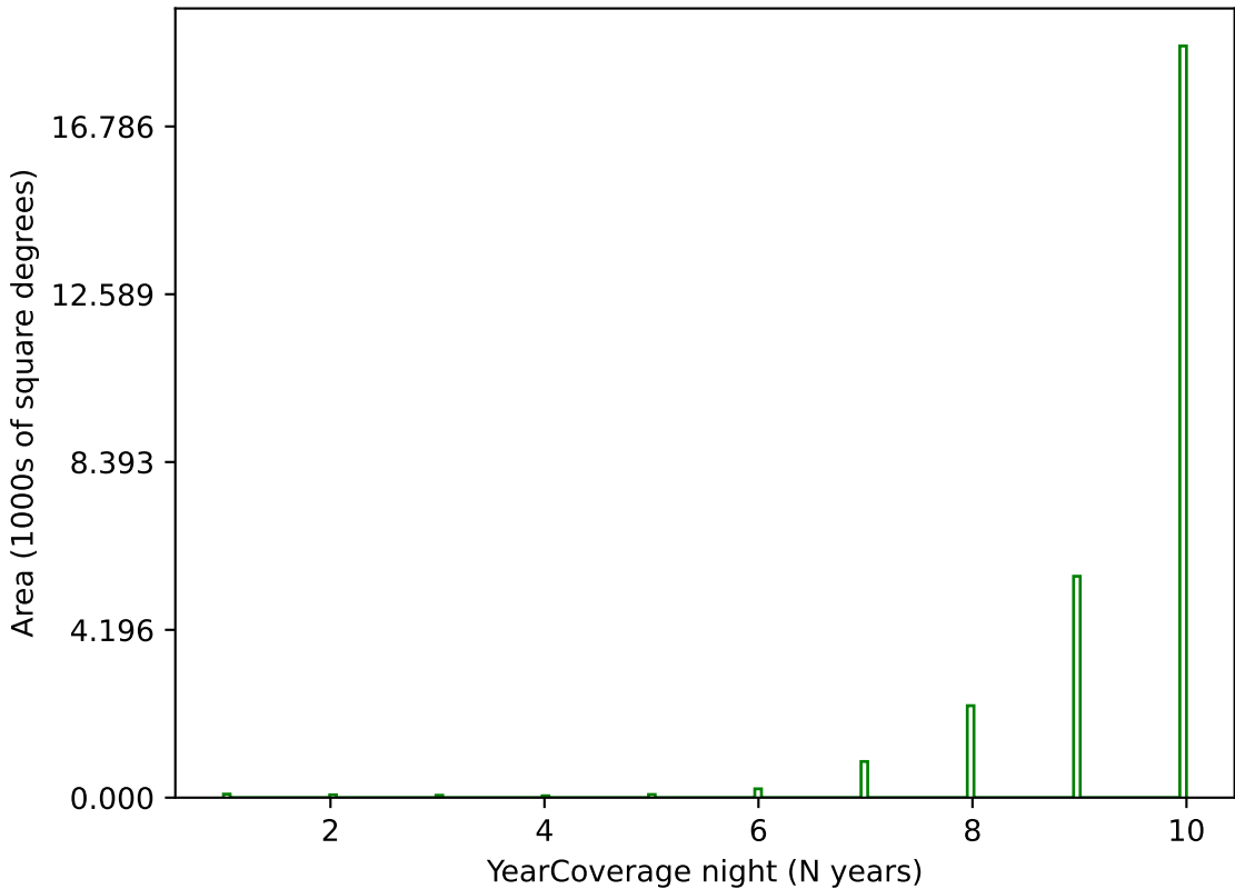
ddf_loaded_half_fl15_v3.4_10yrs g band: YearCoverage night
