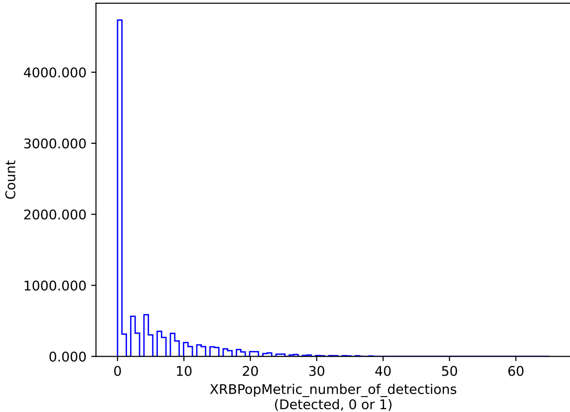
ddf_loaded_half_fl15_v3.4_10yrs : XRBPoMetric_number_of_detections
