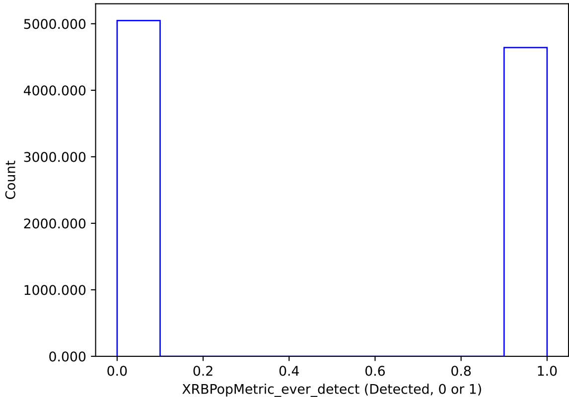
ddf_loaded_half_fl15_v3.4_10yrs : XRBPoMetric_ever_detect
