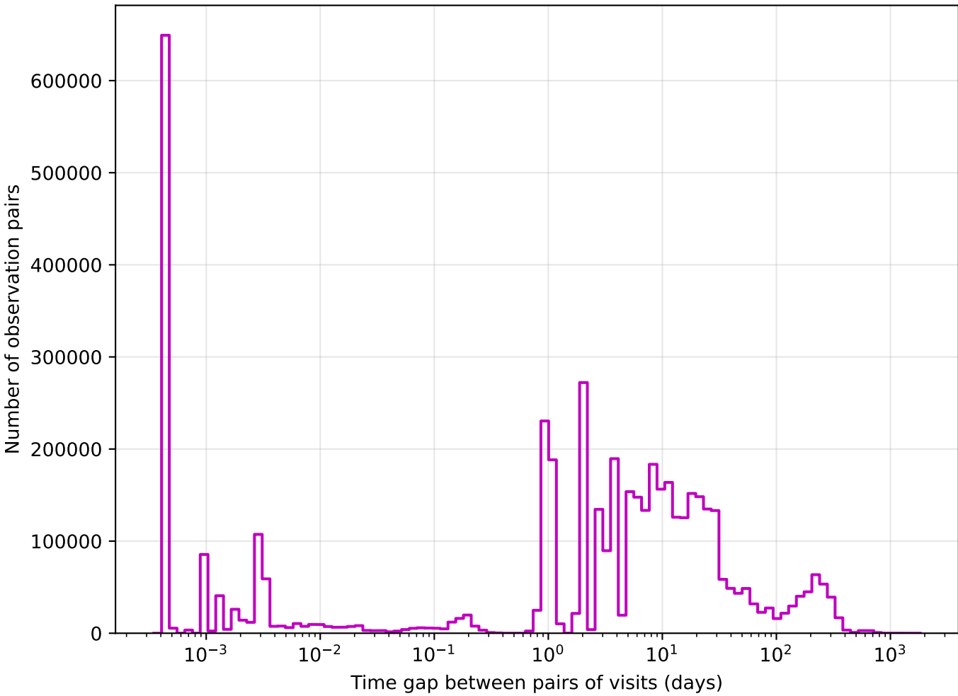
ddf_loaded_half_fl15_v3.4_10yrs z band: Tgaps observationStartMJD
