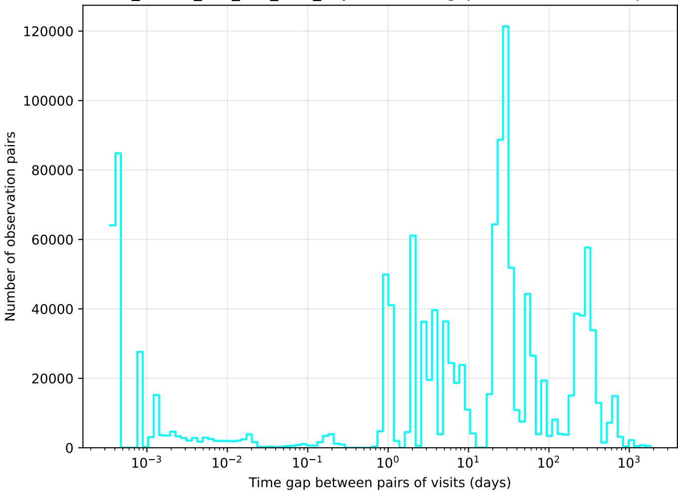
ddf_loaded_half_fl15_v3.4_10yrs u band: Tgaps observationStartMJD
