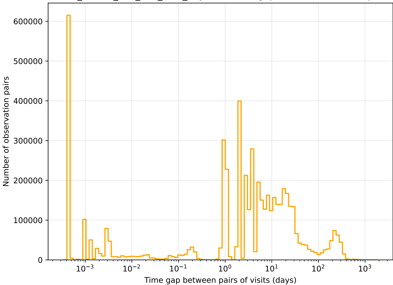
ddf_loaded_half_fl15_v3.4_10yrs r band: Tgaps observationStartMJD
