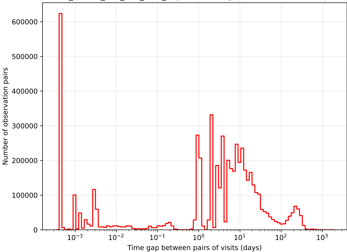
ddf_loaded_half_fl15_v3.4_10yrs i band: Tgaps observationStartMJD
