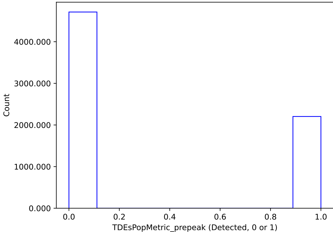
ddf_loaded_half_fl15_v3.4_10yrs : TDEsPopMetric_prepeak
