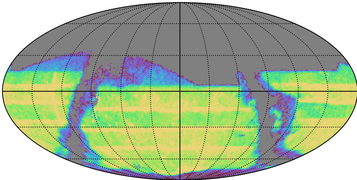
ddf_loaded_half_fl15_v3.4_10yrs : TDC_rate
