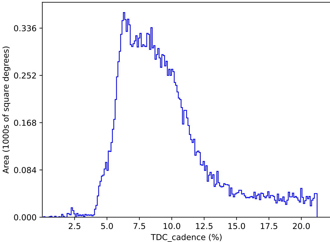
ddf_loaded_half_fl15_v3.4_10yrs : TDC_cadence
