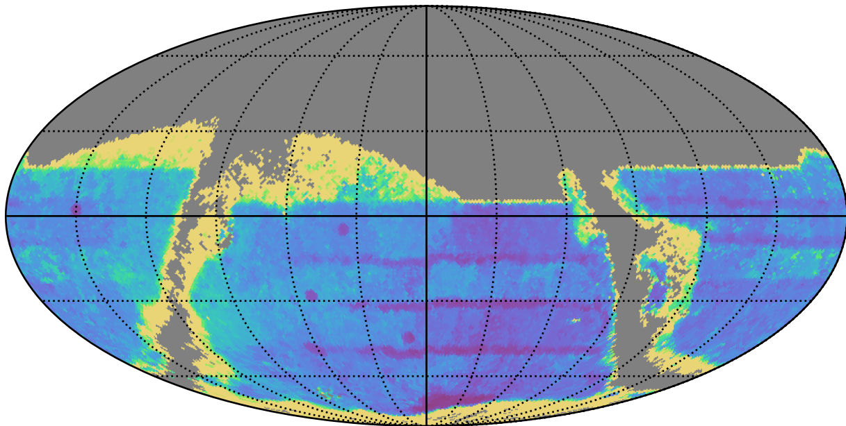
ddf_loaded_half_fl15_v3.4_10yrs : TDC_accuracy
