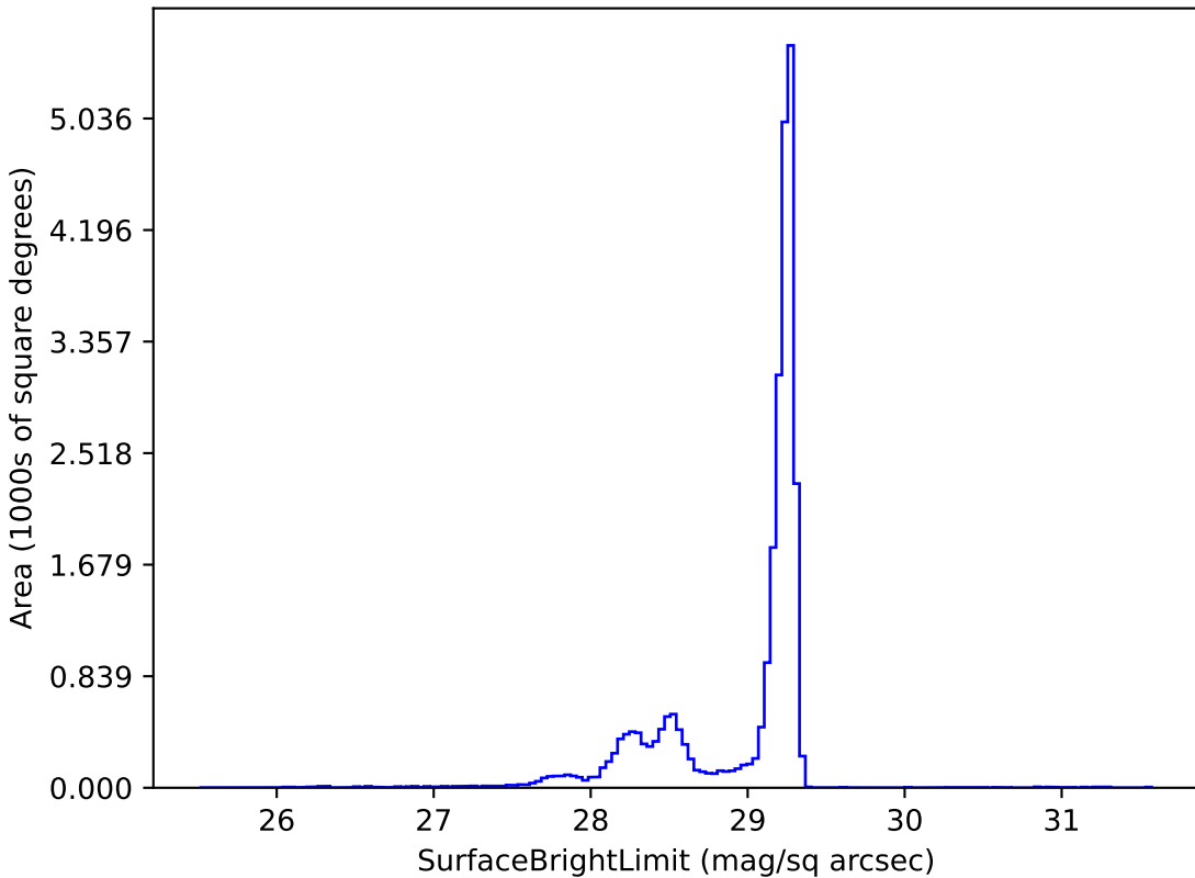
ddf_loaded_half_fl15_v3.4_10yrs z: SurfaceBrightLimit
