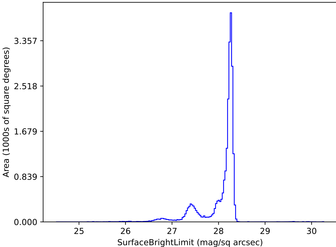
ddf_loaded_half_fl15_v3.4_10yrs y: SurfaceBrightLimit
