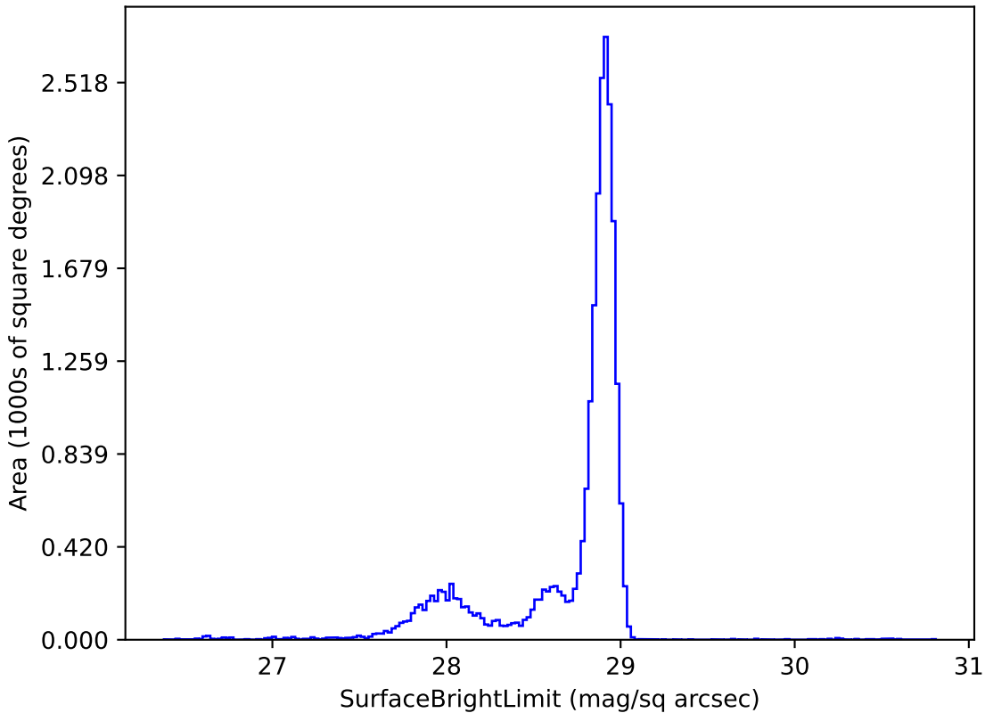
ddf_loaded_half_fl15_v3.4_10yrs u: SurfaceBrightLimit
