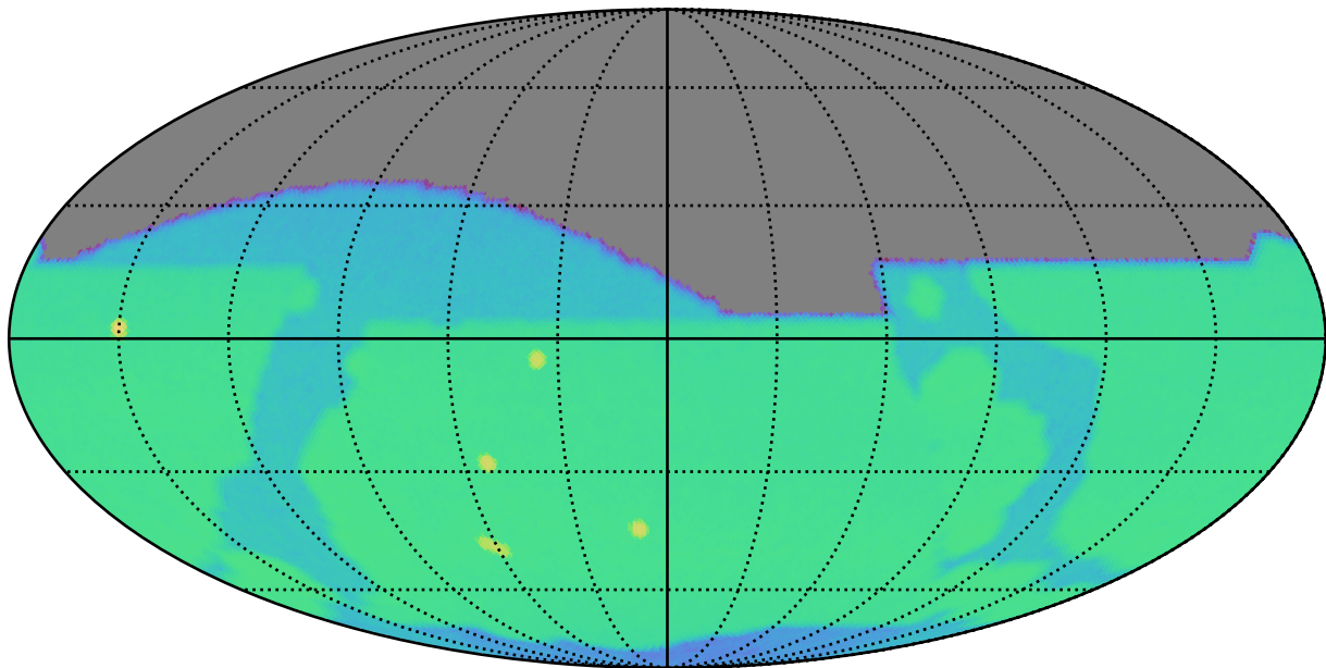
ddf_loaded_half_fl15_v3.4_10yrs r: SurfaceBrightLimit
