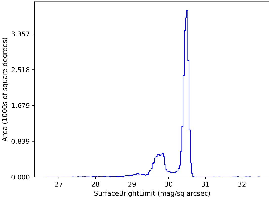
ddf_loaded_half_fl15_v3.4_10yrs r: SurfaceBrightLimit
