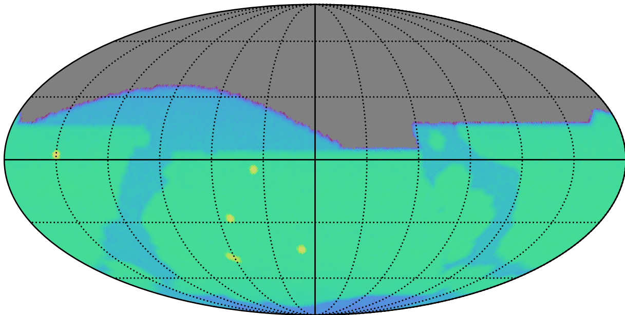
ddf_loaded_half_fl15_v3.4_10yrs i: SurfaceBrightLimit
