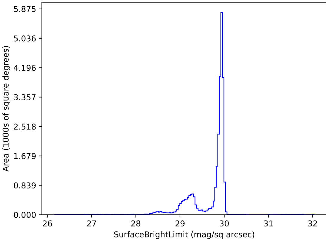
ddf_loaded_half_fl15_v3.4_10yrs i: SurfaceBrightLimit
