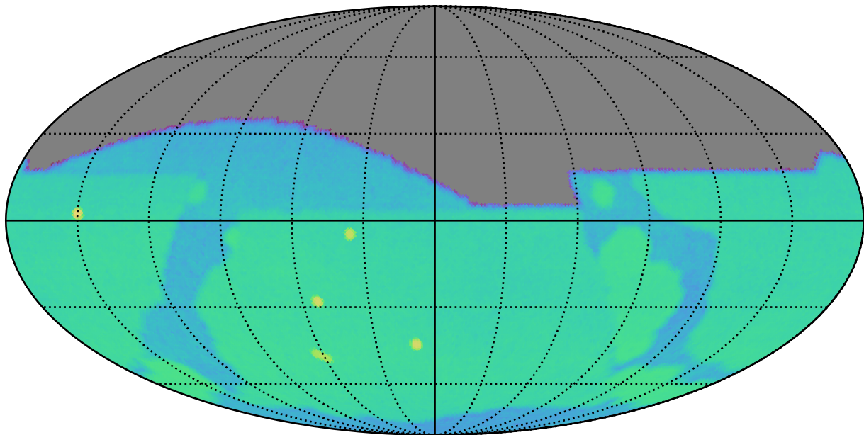
ddf_loaded_half_fl15_v3.4_10yrs g: SurfaceBrightLimit
