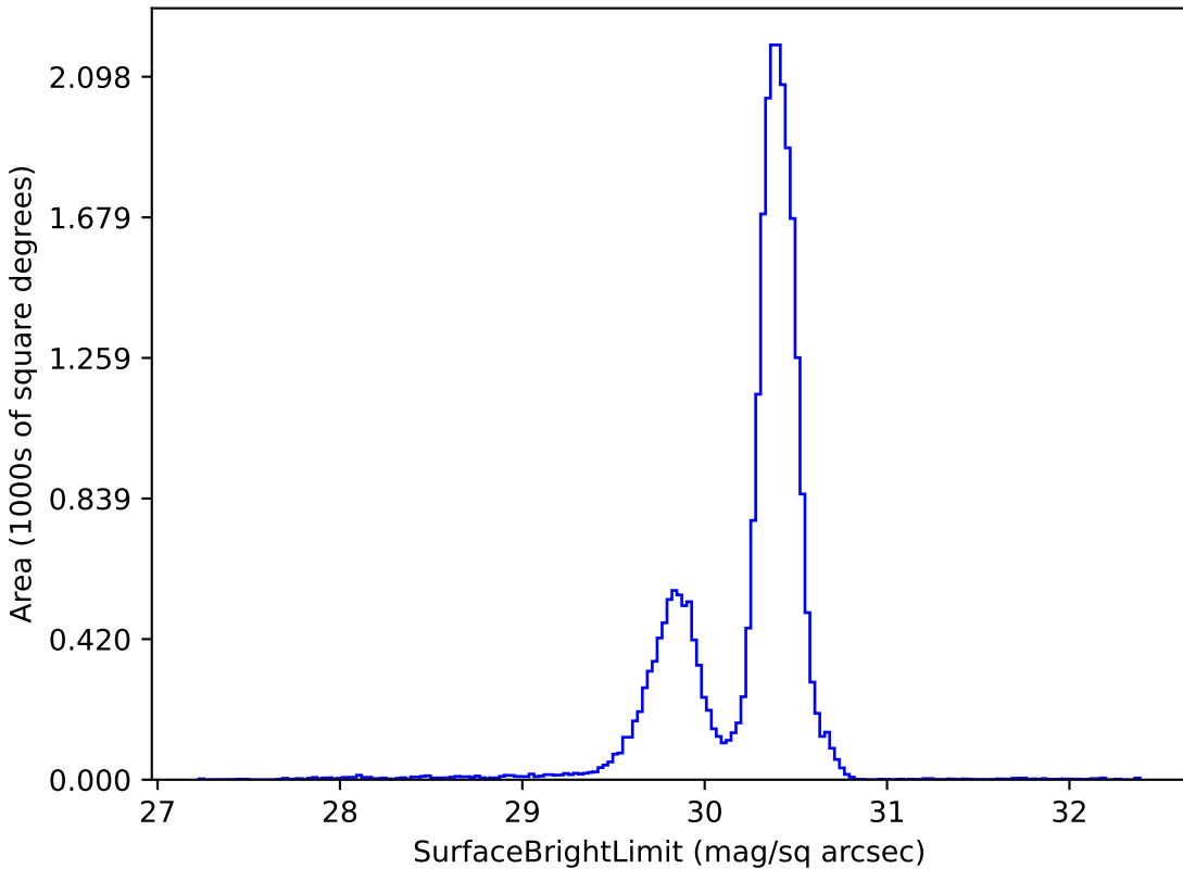
ddf_loaded_half_fl15_v3.4_10yrs g: SurfaceBrightLimit
