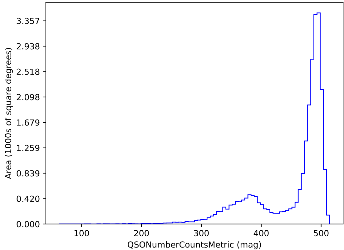
ddf_loaded_half_fl15_v3.4_10yrs z band and non-DD: QSONumberCountsMetric
