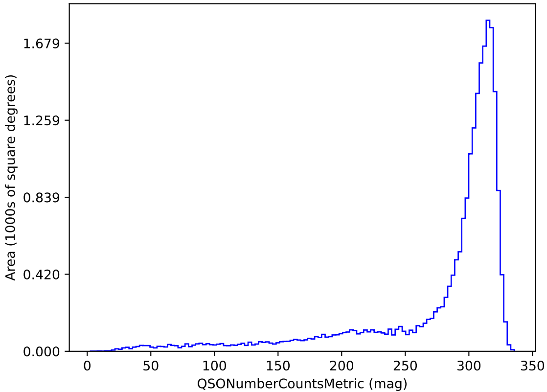
ddf_loaded_half_fl15_v3.4_10yrs u band and non-DD: QSONumberCountsMetric
