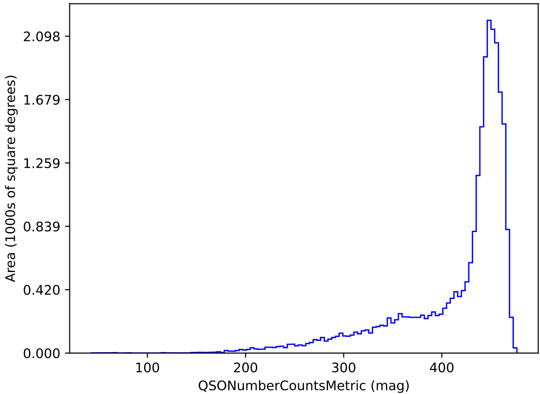
ddf_loaded_half_fl15_v3.4_10yrs g band and non-DD: QSONumberCountsMetric
