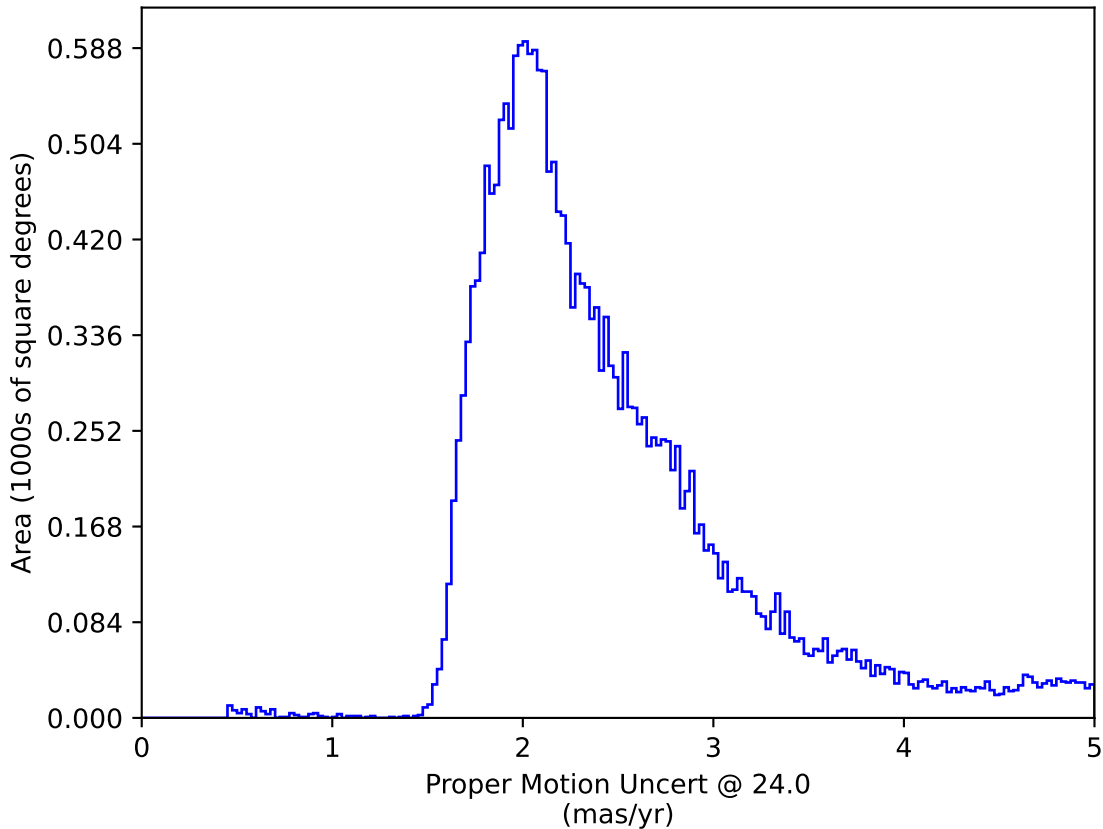
ddf_loaded_half_fl15_v3.4_10yrs : Proper Motion Uncert @ 24.0
