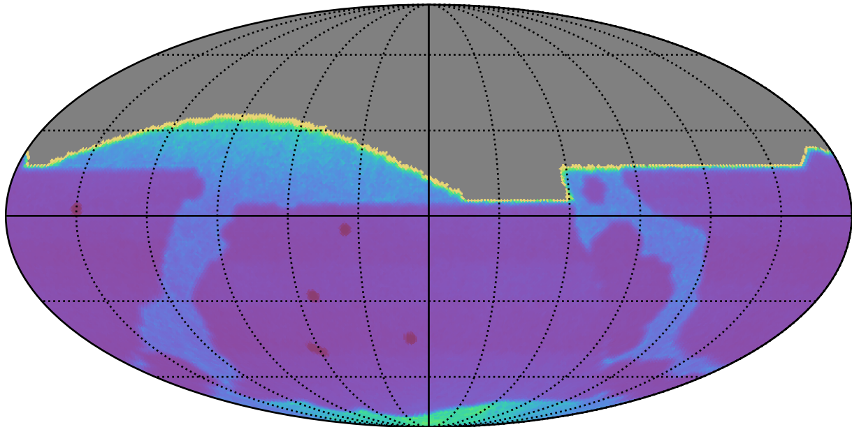
ddf_loaded_half_fl15_v3.4_10yrs : Proper Motion Uncert @ 20.5
