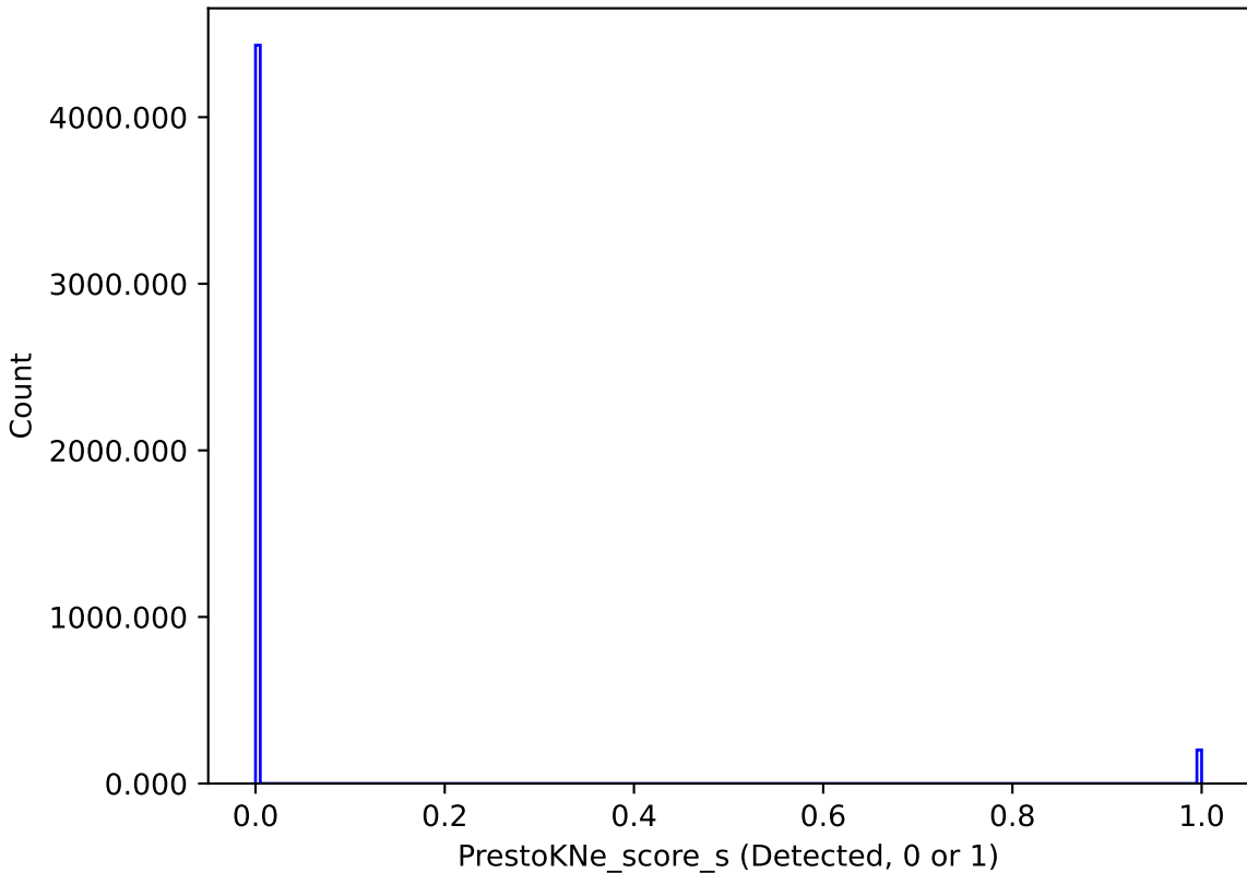
ddf_loaded_half_fl15_v3.4_10yrs : PrestoKNe_score_s
