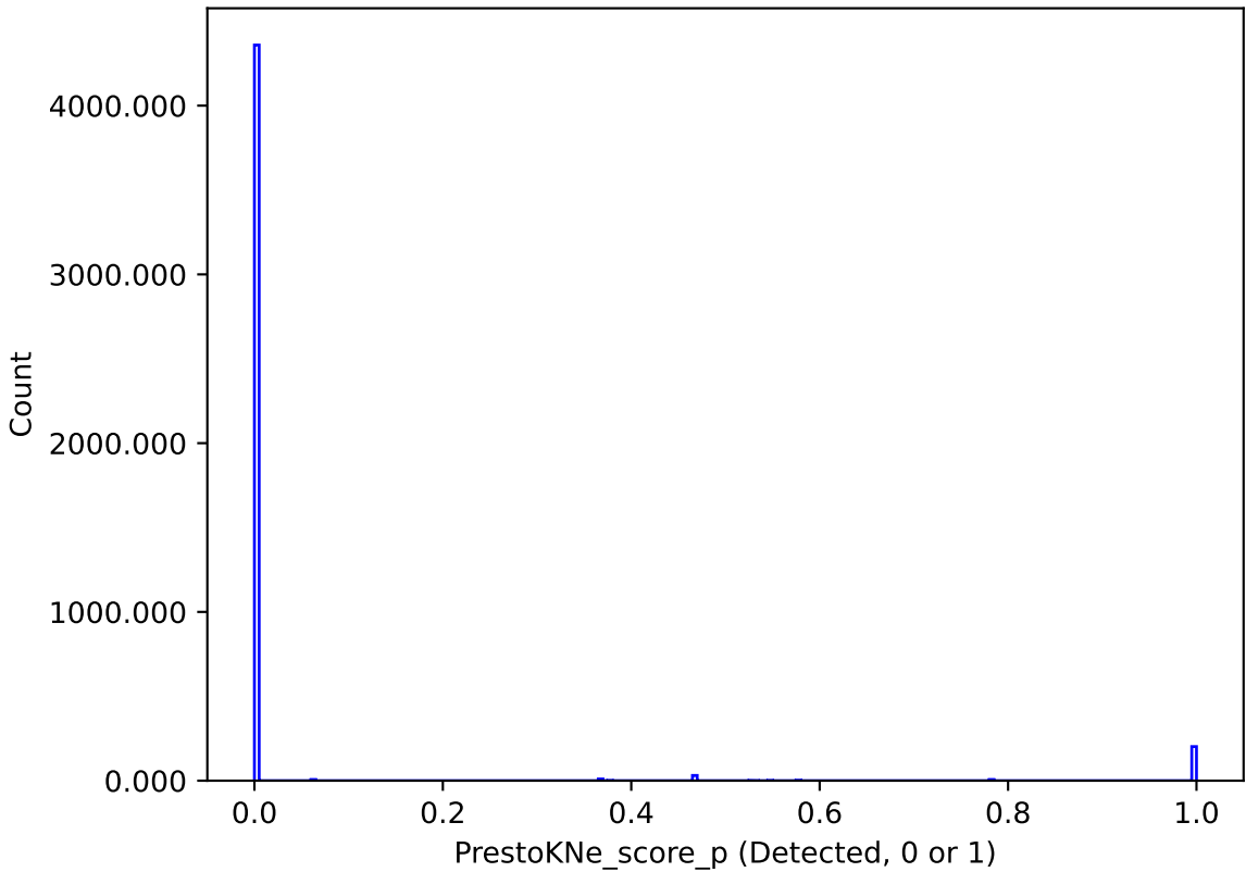
ddf_loaded_half_fl15_v3.4_10yrs : PrestoKNe_score_p
