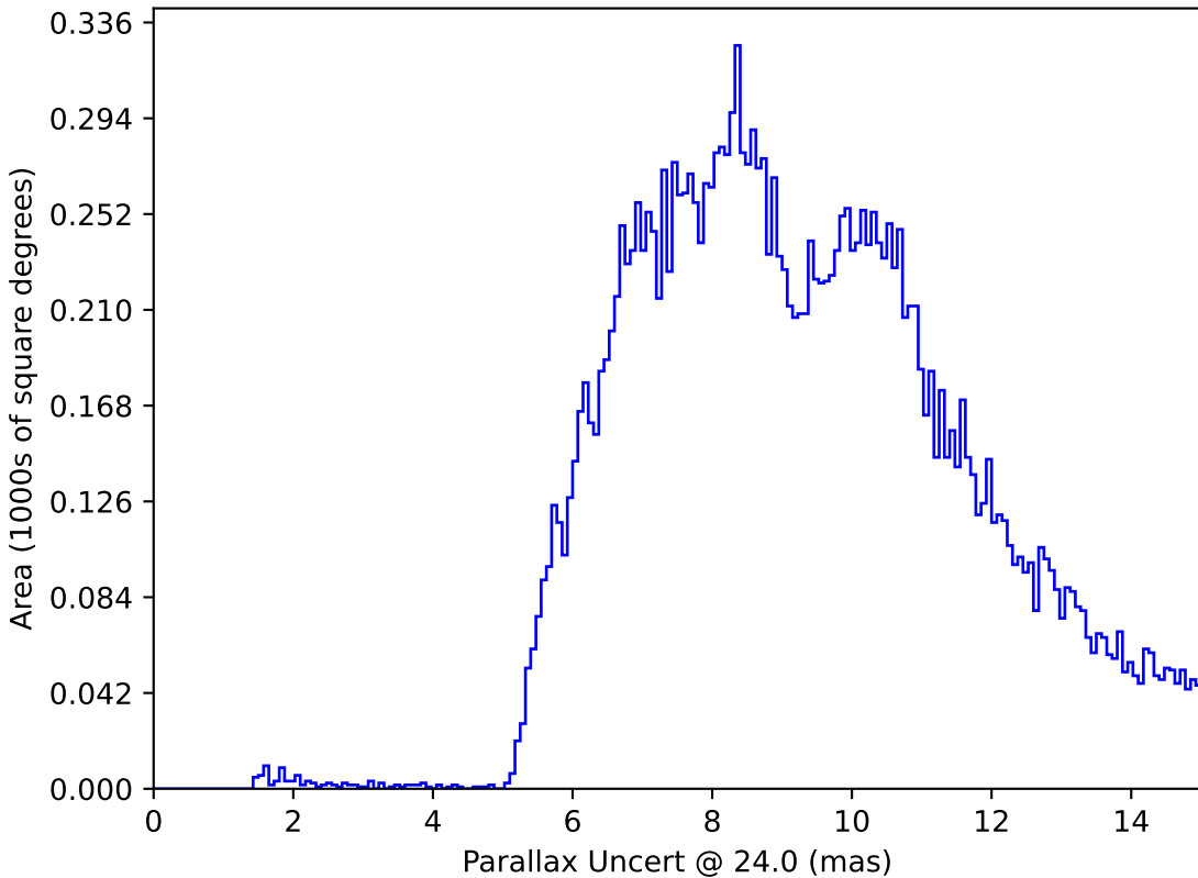
ddf_loaded_half_fl15_v3.4_10yrs : Parallax Uncert @ 24.0
